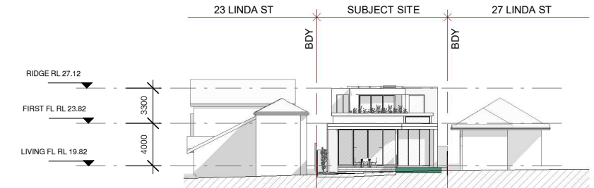
2 EAST ELEVATION. 1 : 500
