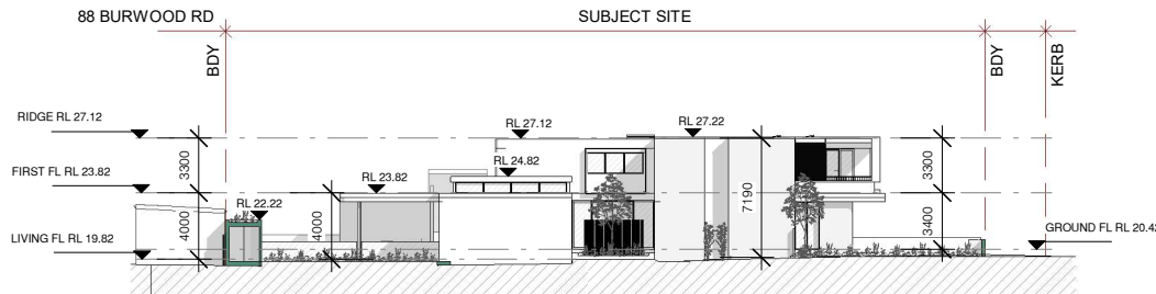
4 NORTH ELEVATION 1 : 500
