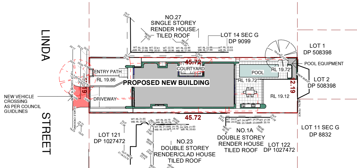
1 NOTIFICATION PLAN 1 : 500
