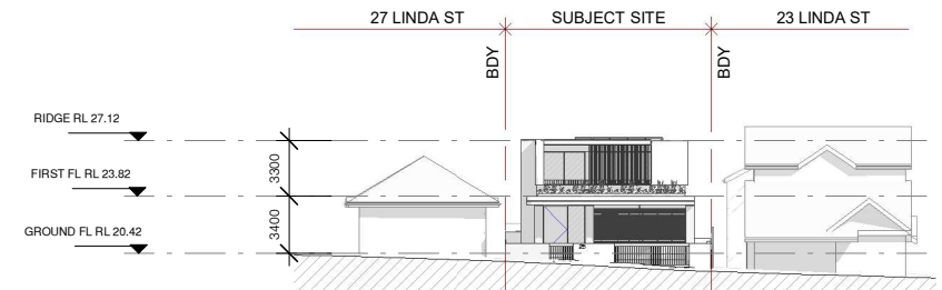
3 WEST ELEVATION - LINDA ST 1 : 500
